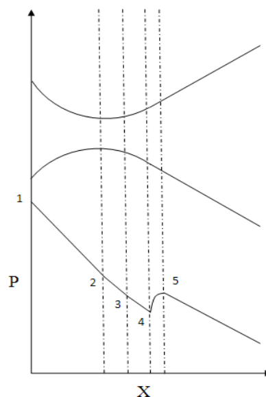
Figure 2. Axial pressure distribution in nozzle with condensation.
