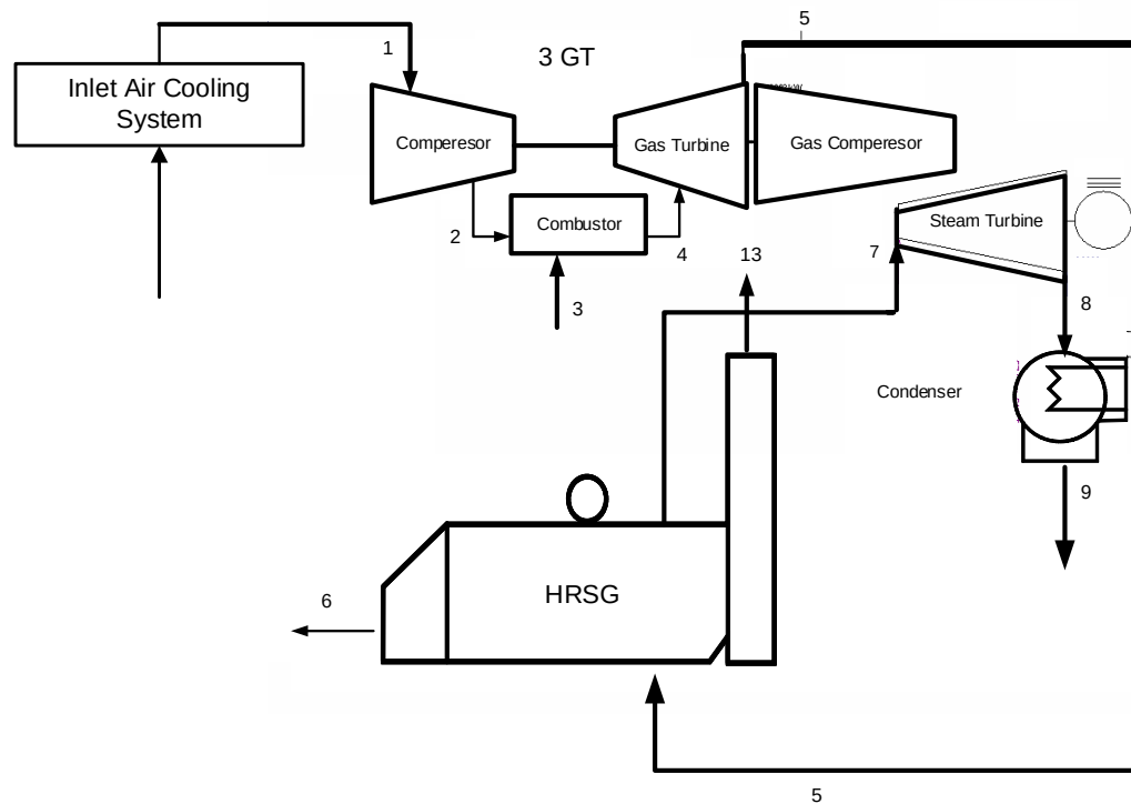
Figure 1. The Schematic of this Proposed Combined Cycle
