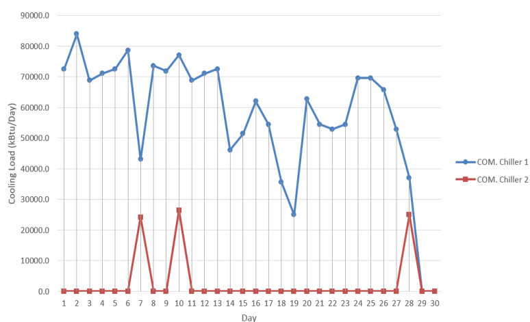
Figure 16. Vapor compression Chillers Cooling load in September
