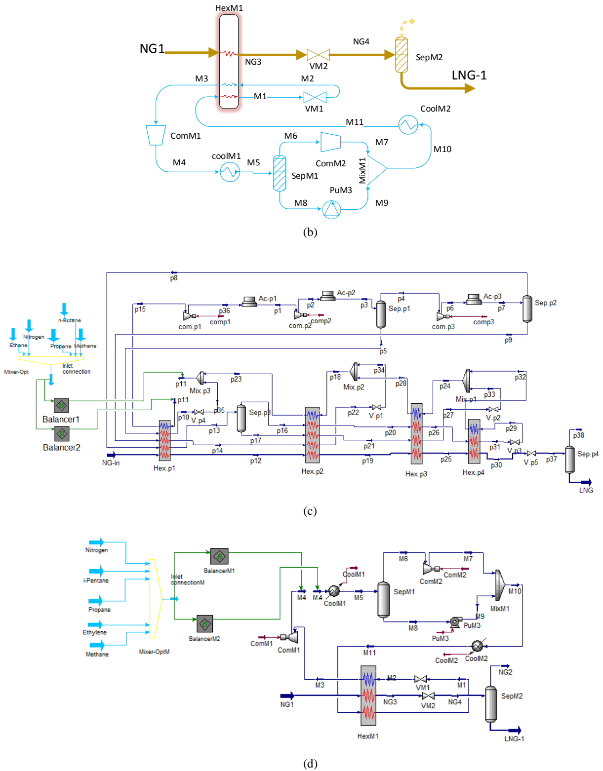
Fig. 2. LIMUM3 and PRICO process diagrams ;(a) LIMUM3 flow diagram, (b) PRICO flow diagram, (c) LIMUM3 HYSYS diagram, (d) PRICO HYSYS diagram.
