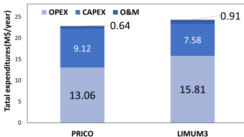
Fig. 10. Comparison of annual CAPEX, OPEX, and O&M expenses for PRICO and LIMUM3 cycles in optimized case.
